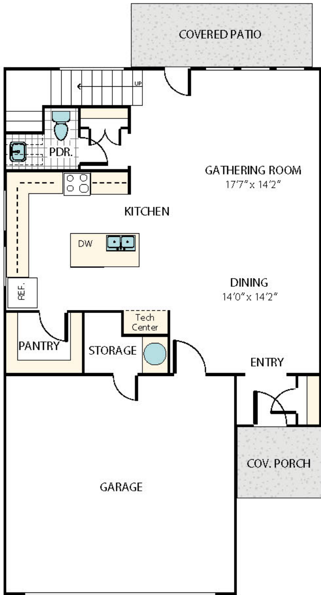
Main Level Elevation C
