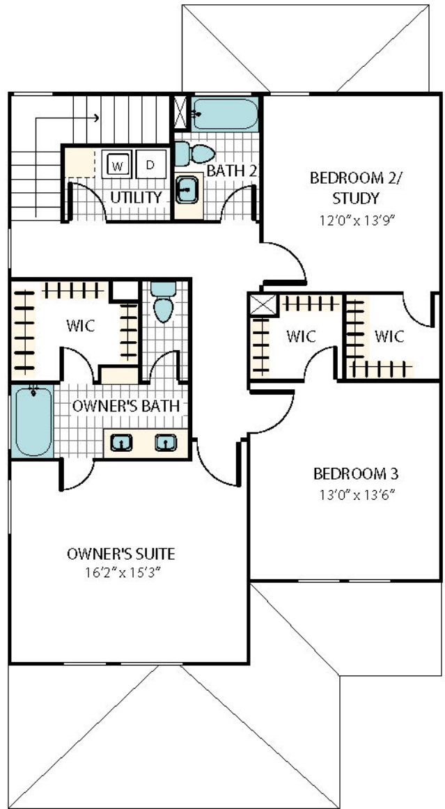
Upper Level Elevation A, B, C
