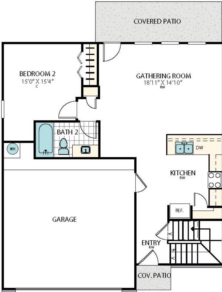
Main Level Elevation G
